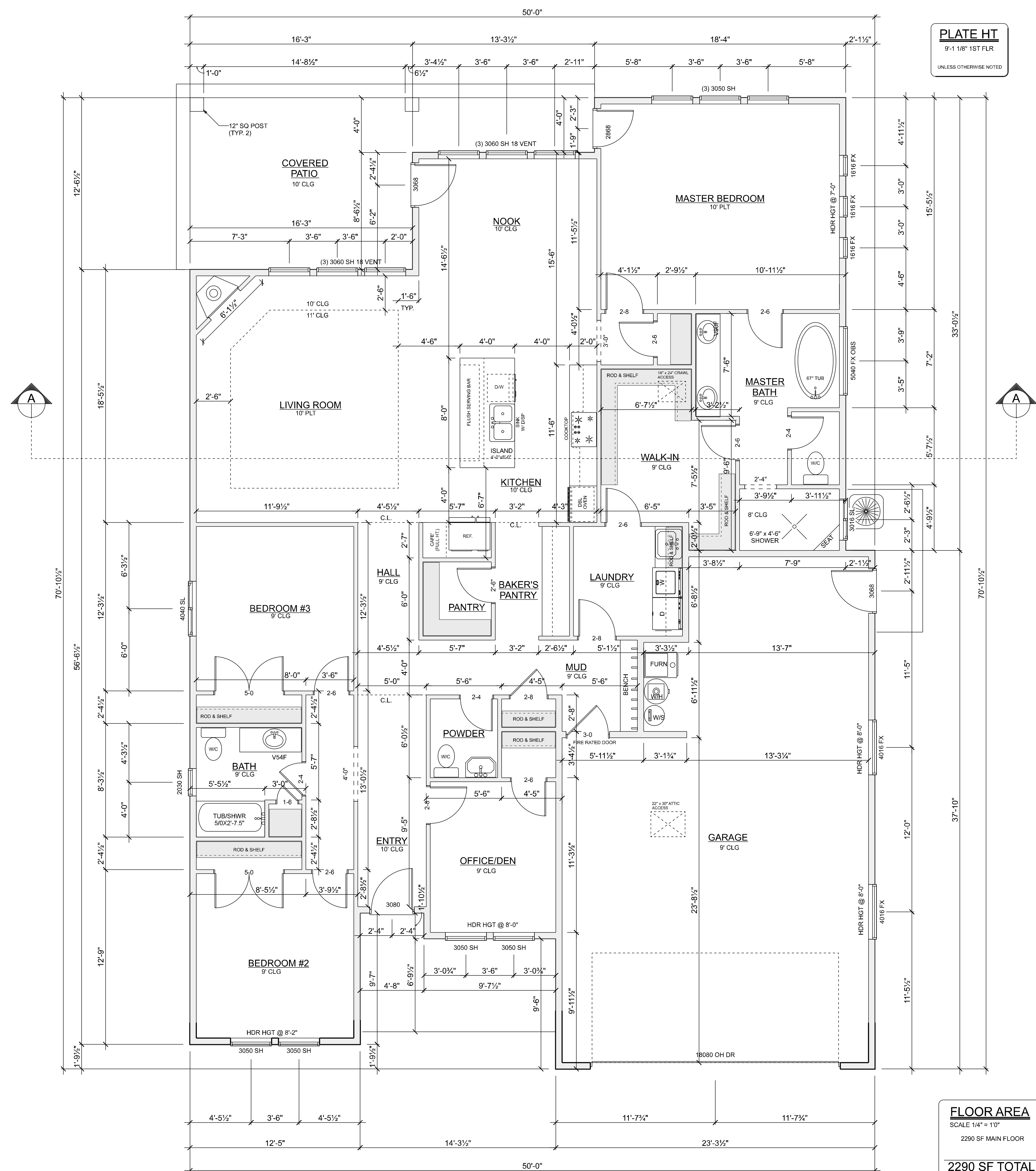
FLOOR PLAN - MAIN SCALE : 1/4" = 1'-0" (FULL SIZE PLANS)
